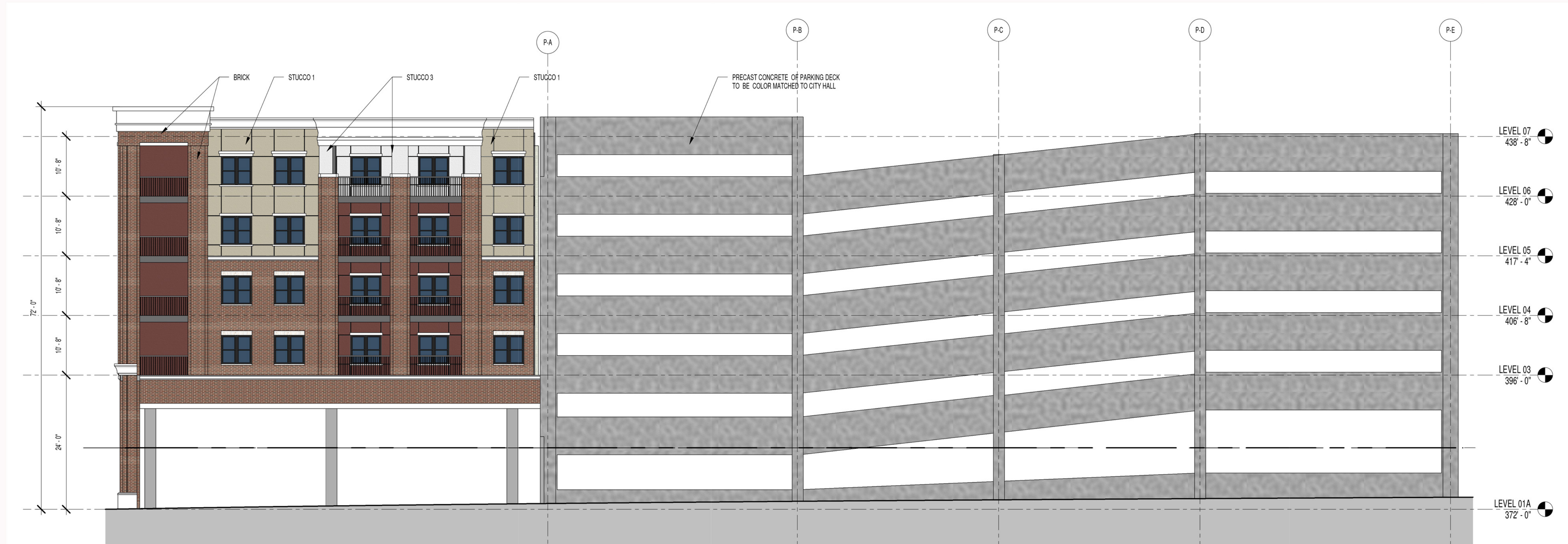
EAST ELEVATION
