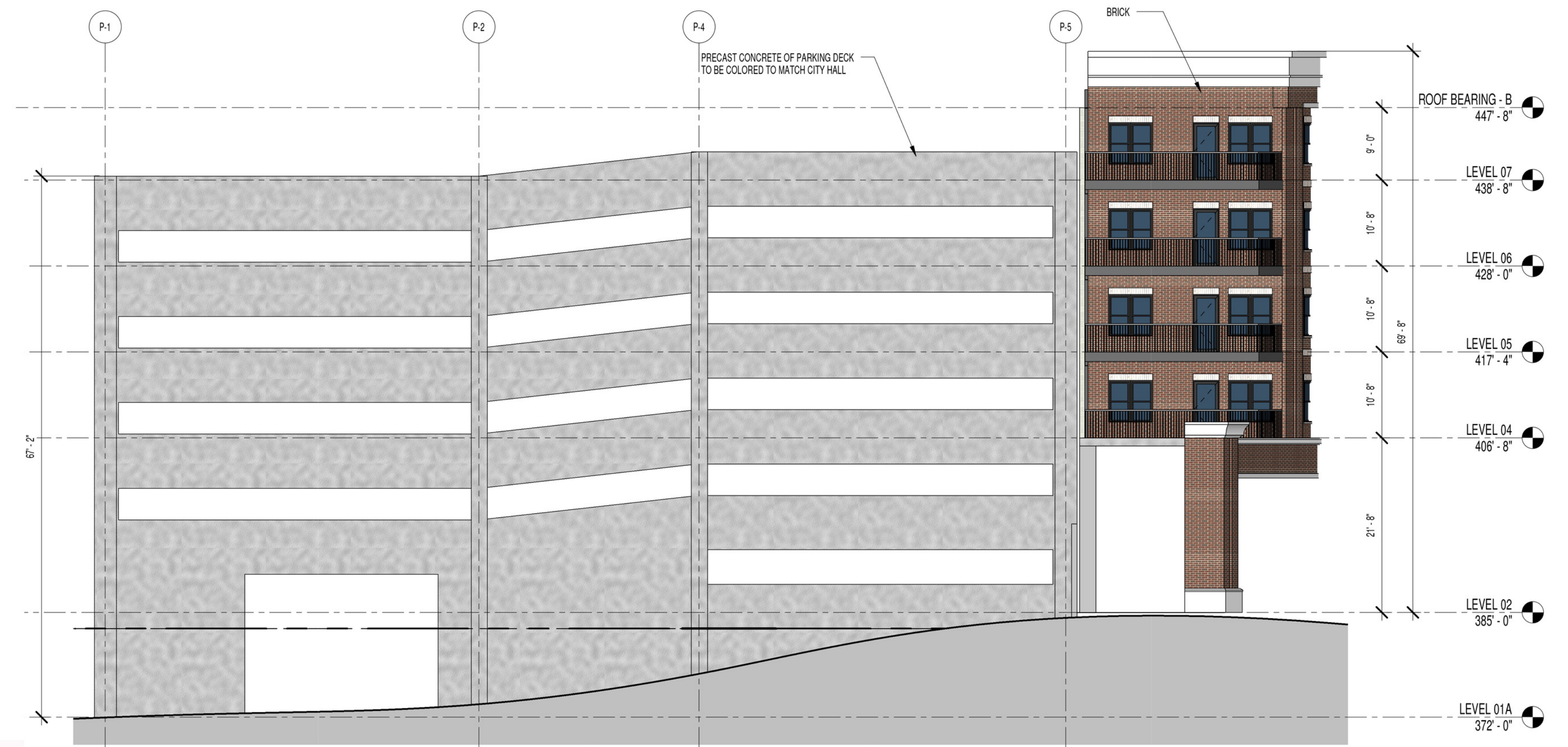
NORTH ELEVATION
